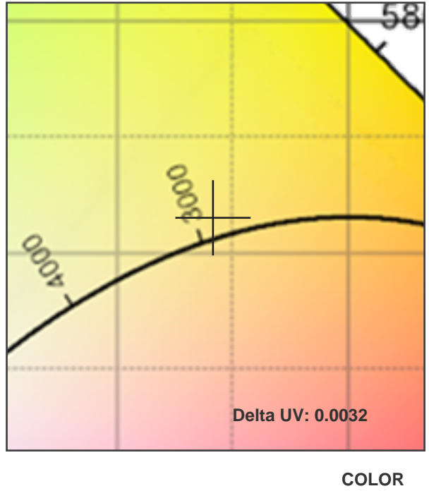
CRI: 77.8 (R1-R8)
