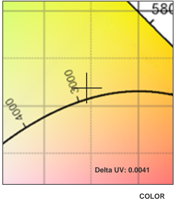
CRI: 76.8 (R1-R8)
