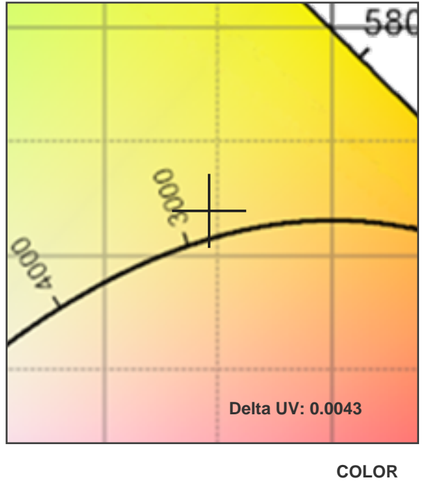
CRI: 76.7 (R1-R8)
